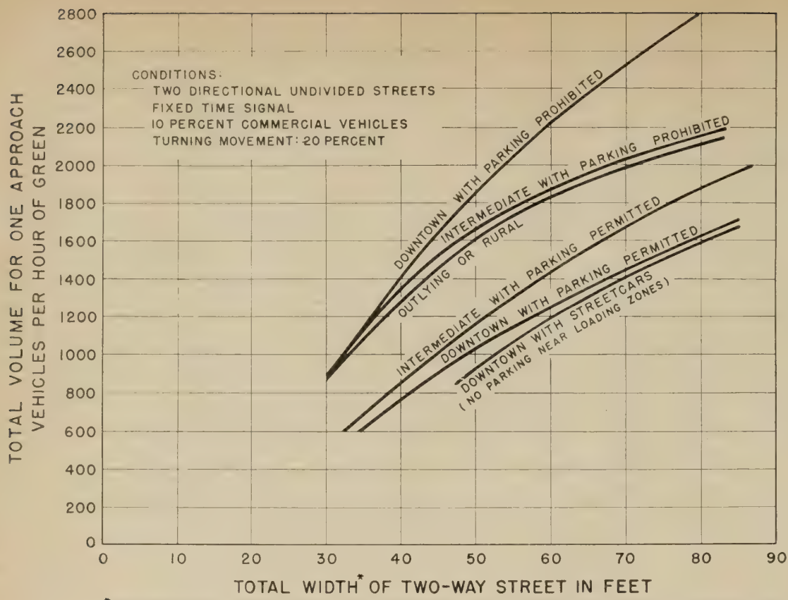
Figure 24.—Average reported intersection capacities for two-way streets by type of area and parking regulation.
